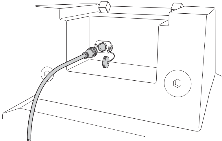
Figure 2-10 External device connection at rear of sampler
