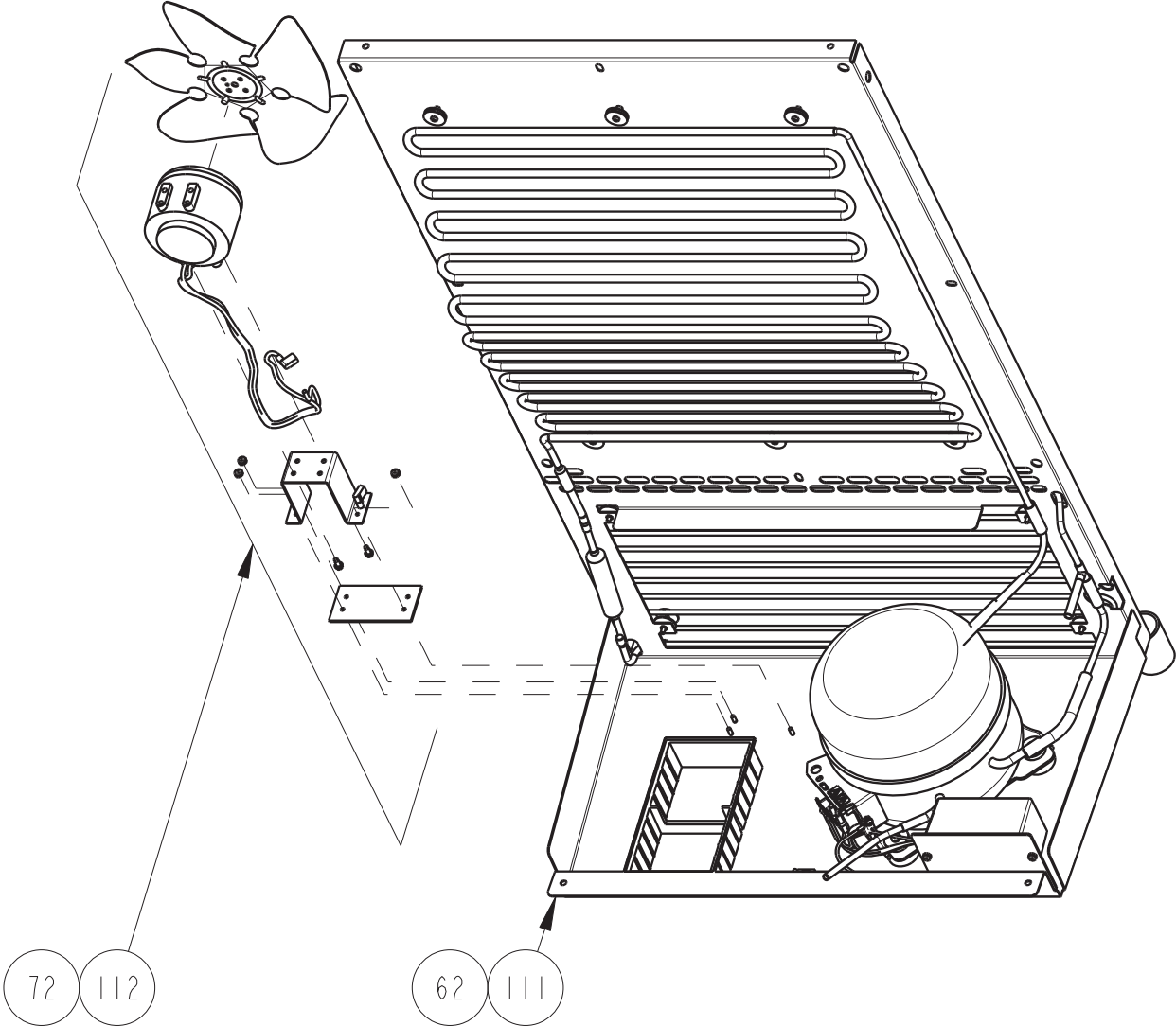
117V VIEW
