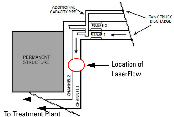
Overhead view of the measurement area
