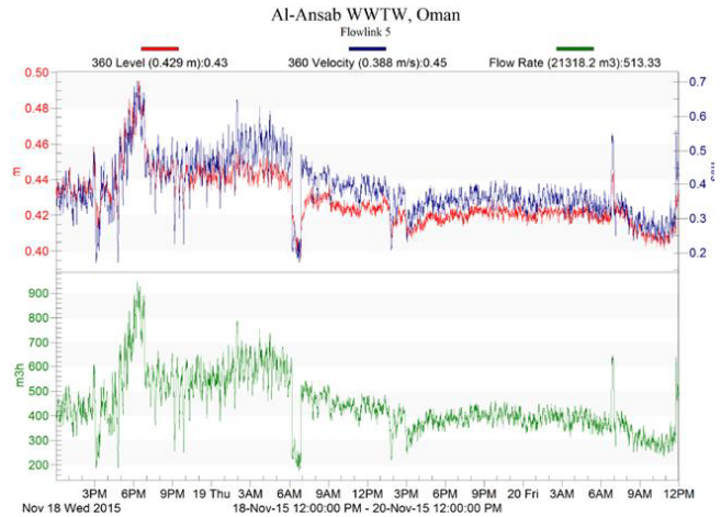
Measurement results displayed using Flowlink® software
